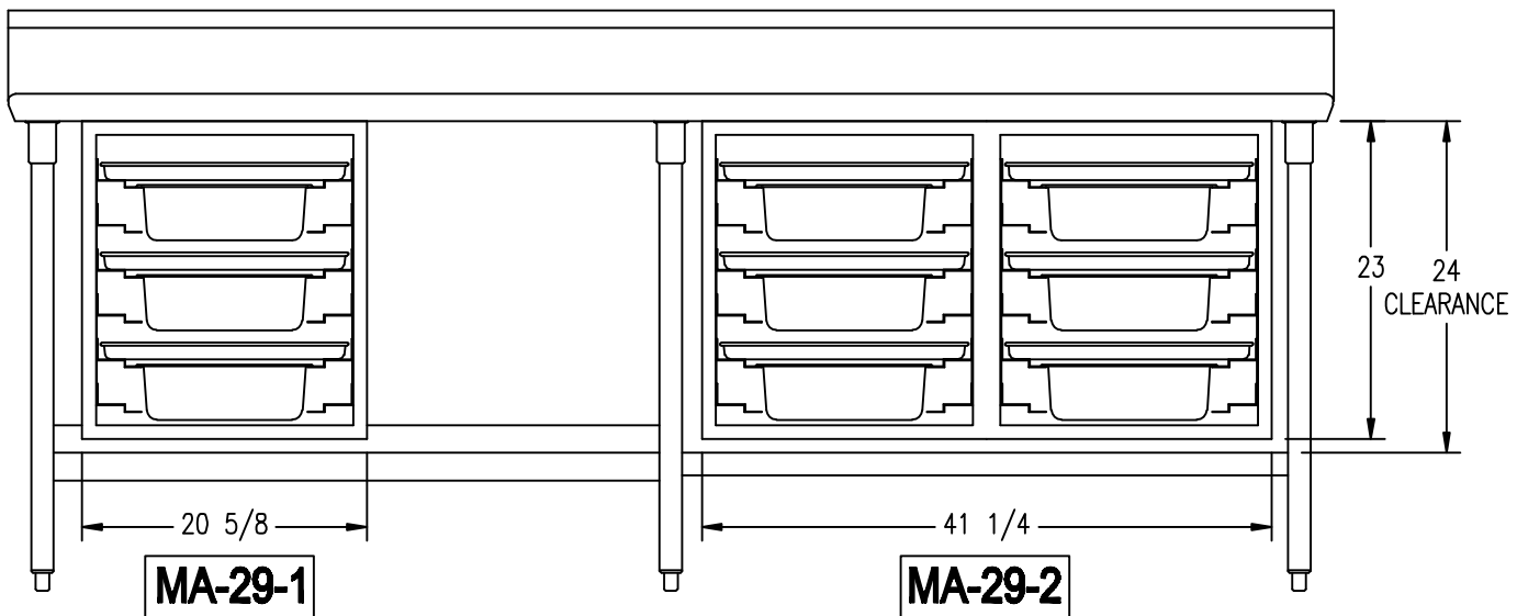
ELEVATION VIEW FOR MOUNTING PAN RACK ASSEMBLIES
