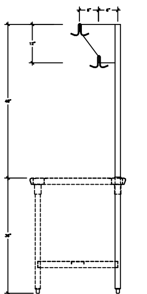
Model # APR-2T series Double Bar Pot Rack Assembly
