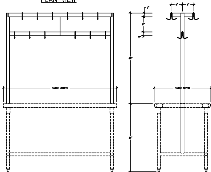
Model # APR-3T series Triple Bar Pot Rack Assembly
