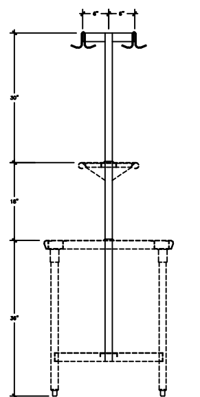
Model # APR-4T series Double Bar Pot Rack Assembly
