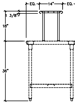
AOS-3S SERIES
