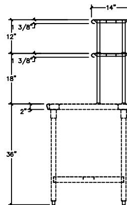
AOS-4D SERIES
