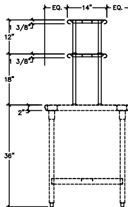
AOS-3D SERIES
