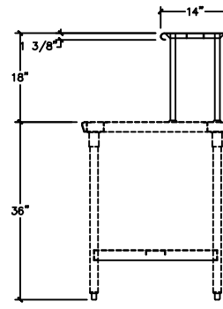
AOS-4S SERIES
