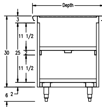
SECTION OPTIONAL INTERMEDIATE SHELVING
