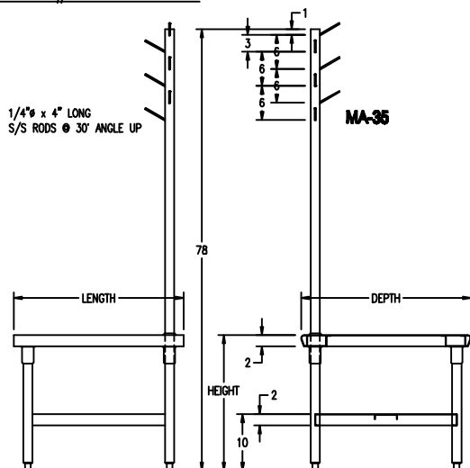
ELEVATION VIEW
