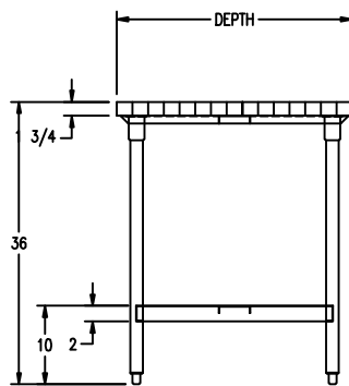
SECTION
