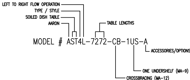
MODEL # AST4L-7272-CB-US SERIES CORNER SOILED DISH TABLE LEFT TO RIGHT OPERATION
