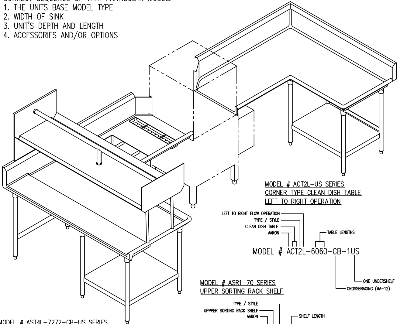
MODEL # AST4L-7272-CB-US SERIES CORNER SOILED DISH TABLE LEFT TO RIGHT OPERATION
