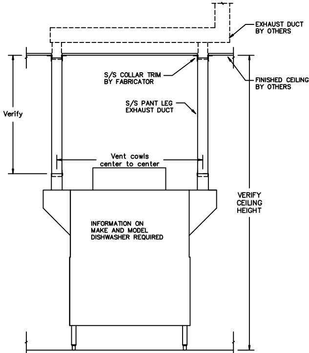
MODEL # AEV1-SERIES ELEVATION
