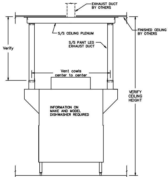
MODEL # AEV2-SERIES ELEVATION
