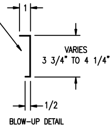
BLOW-UP DETAIL
