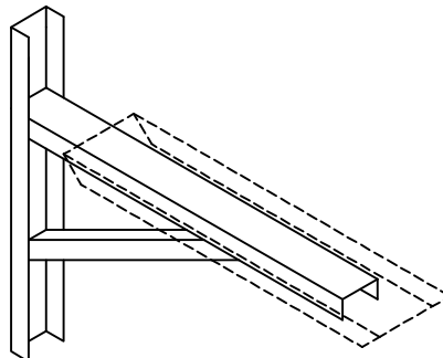
CANTILEVER BRACKET ITEM NO. UBA-32
