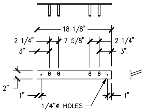
TWO HOLDER MOP BRACKET
