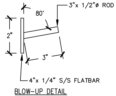
BLOW-UP DETAIL
