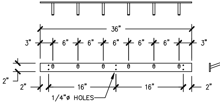
FLOOR MAT HANGING BRACKET
