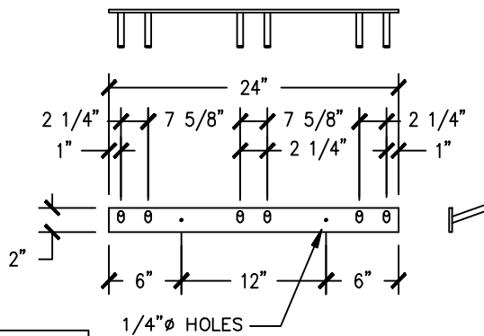
THREE HOLDER MOP BRACKET
